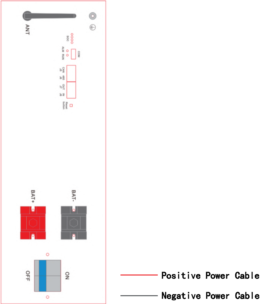
Fig. 6-3GND Cable Connection Diagram
