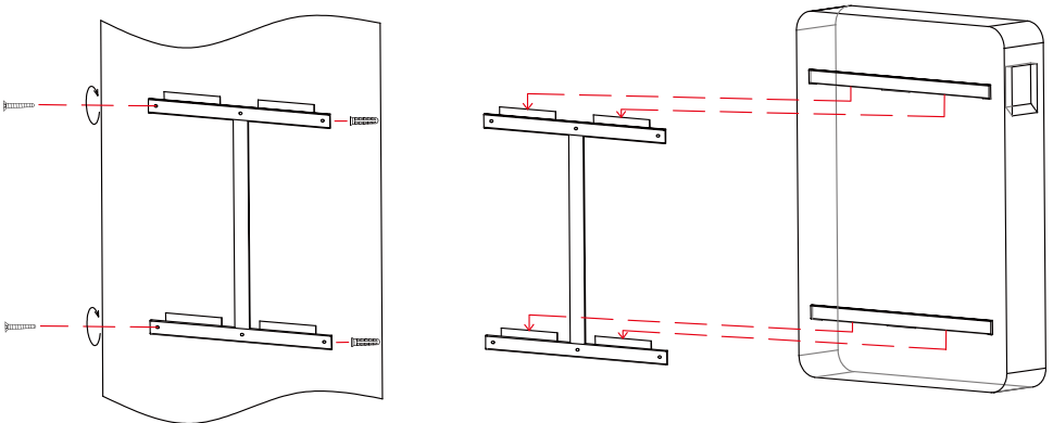
Fig.6-2 Fix the Battery to the Wall
