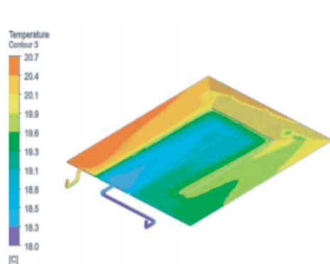
Cloud map of the coolant temperature field
