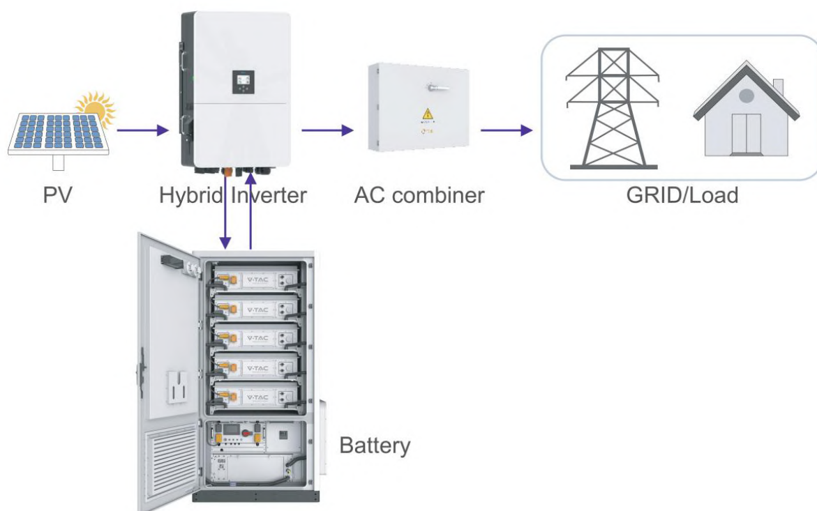
Figure2-1 Energy storage system constitution
