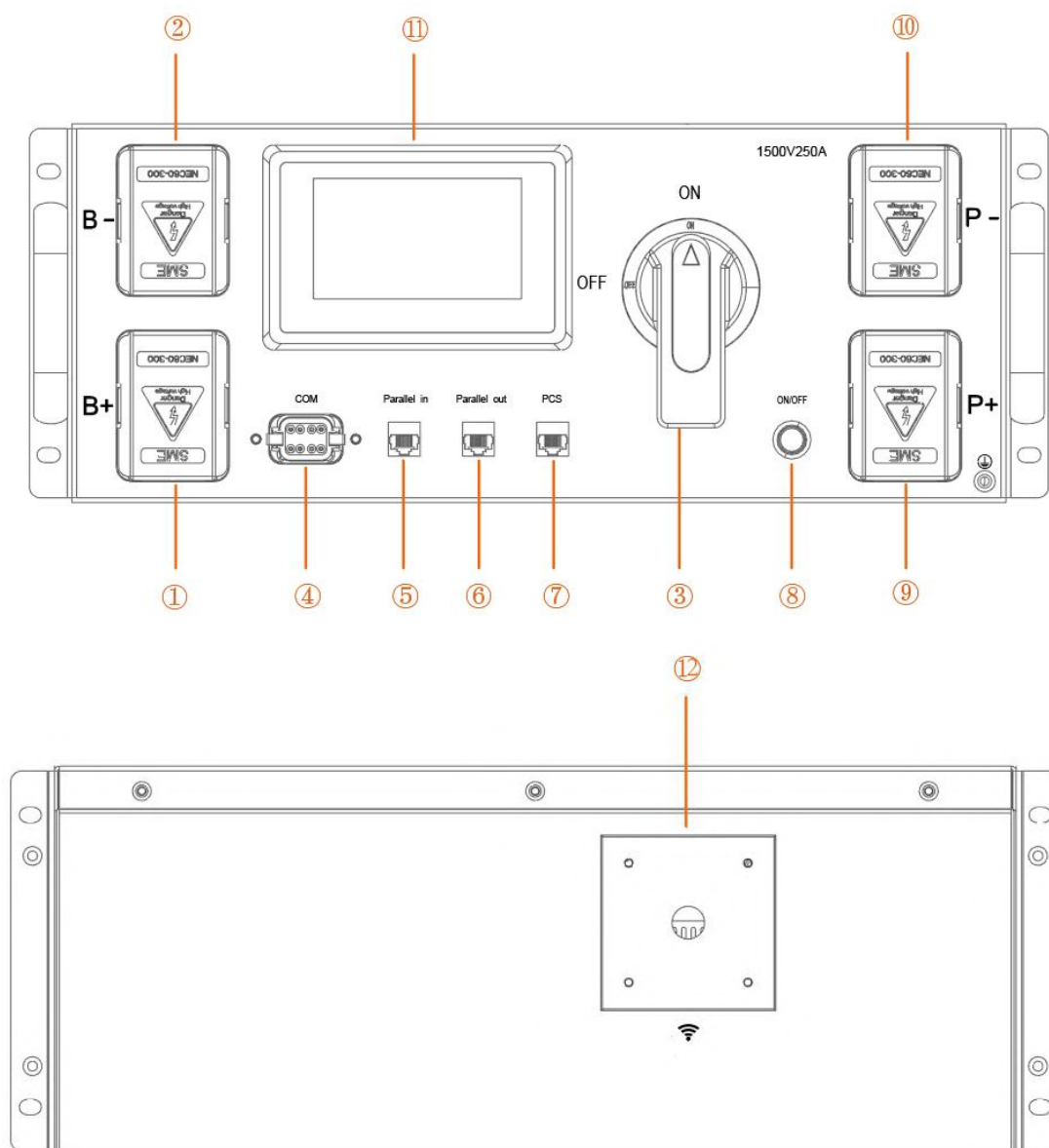
Figure2-6 Structure layout
