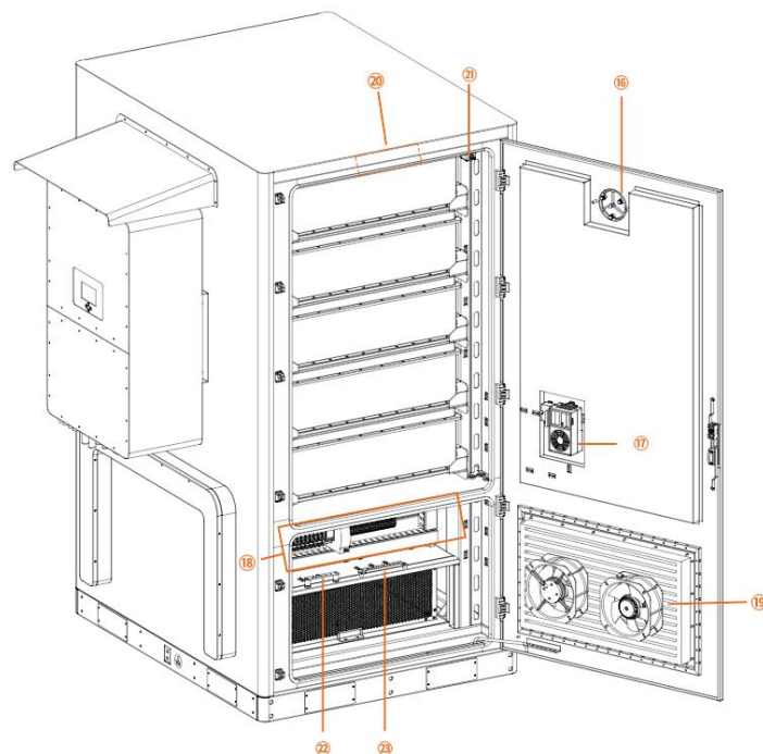
Figure2-4 Structure layout (Open the back door)
