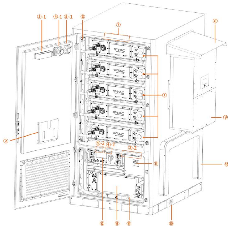
Figure2-3 Structure layout (open the front door)
