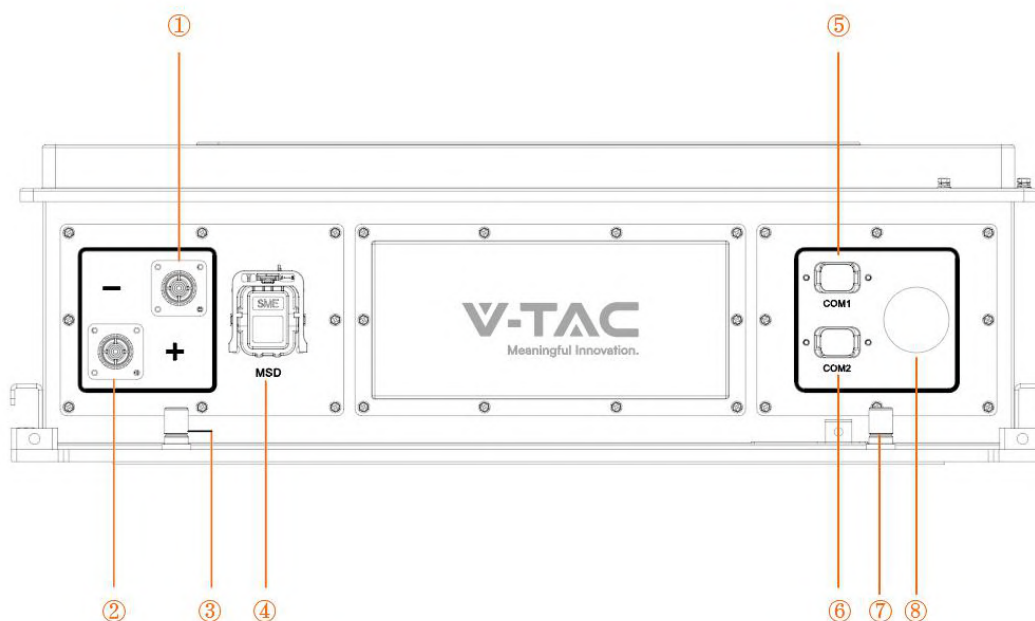
Figure2-5 Structure layout
