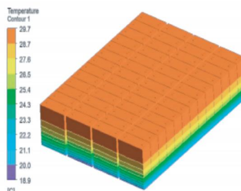
Battery temperature field cloud map
