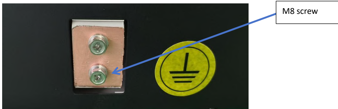
Figure2-11 Cabinet grounding terminals diagram
