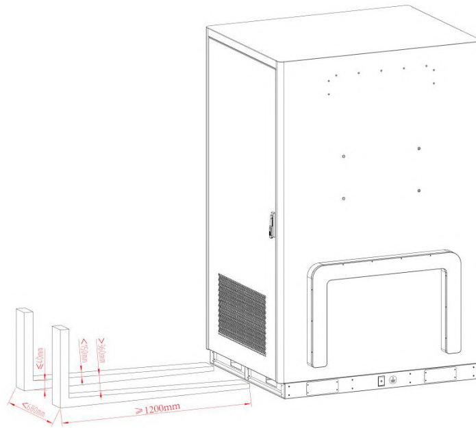
Figure3-6 Forklift transportation diagram (unit: mm)
