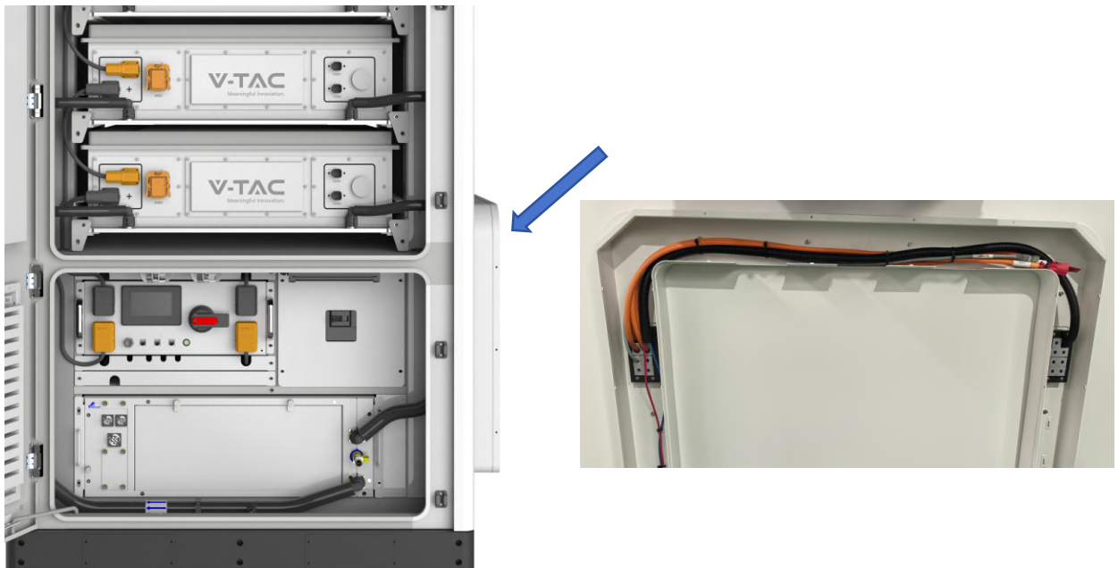
Figure2-12 Inside the wire trough
