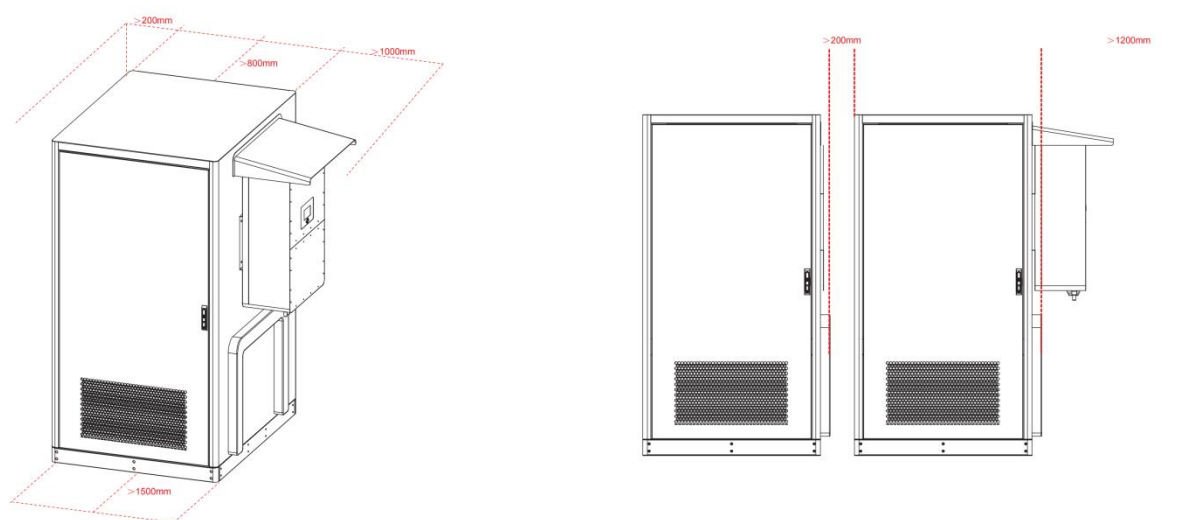
Figure3-5 Installation space (unit: mm)
