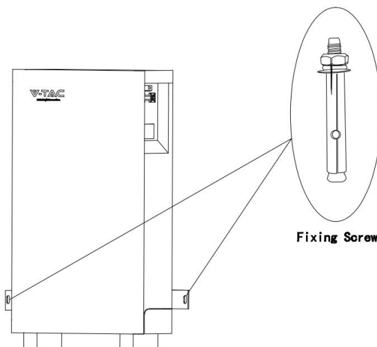
Fig.6-3 Fix the Battery to the Wall
