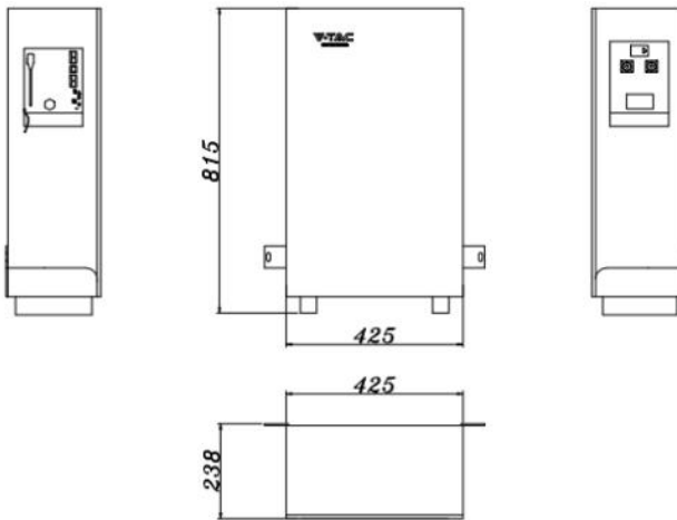
Fig. 5-1 Product Dimensions
